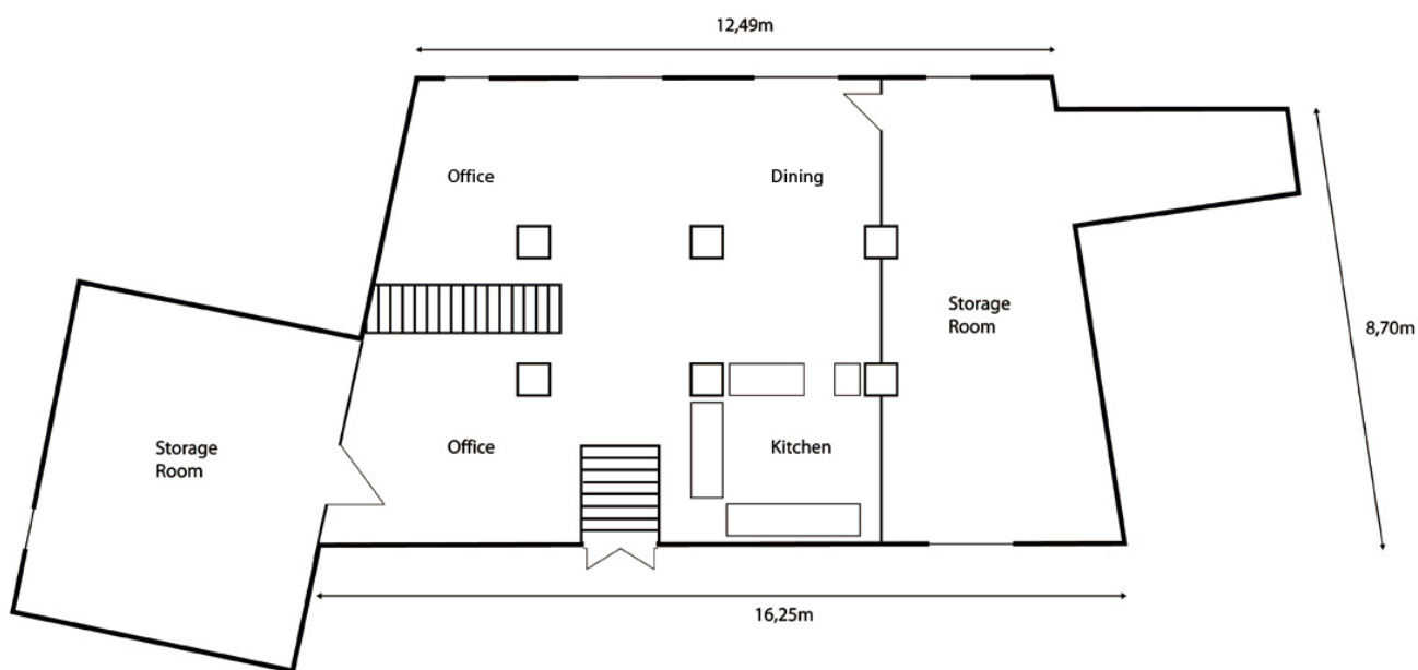
GRUNDRISS BASEMENT
